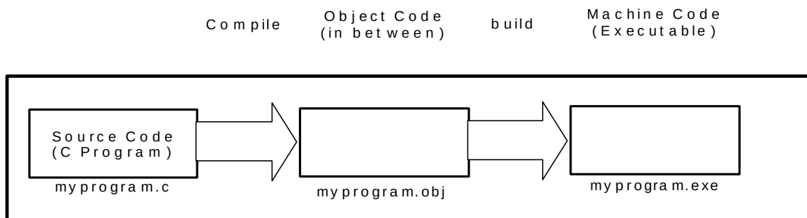
Fig 1.0. Compilation Process
