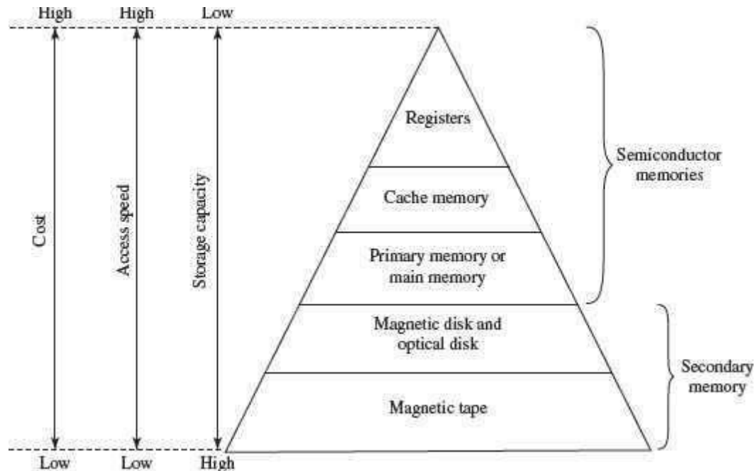
Figure 1.9 Memory hierarchy
